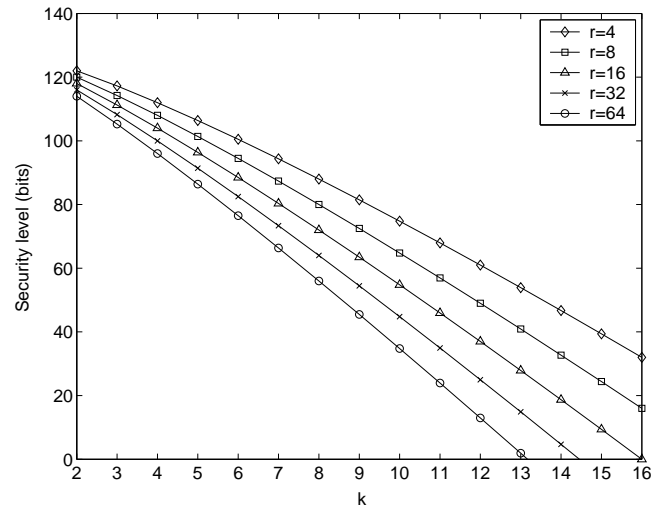
Figure 10 Security level as a function of k .
