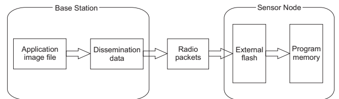
Figure 1 Code dissemination process.
