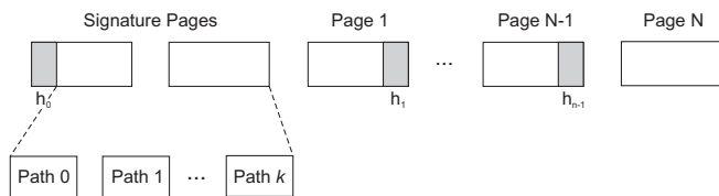
Figure 11 Partitioning of the program image into pages before the dissemination into the network. This also shows the order at which a mote receives the signature, the pages and their hash values. Verification of the signature is possible by storing only one path at the time.
