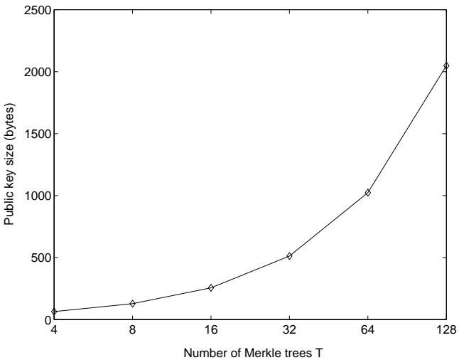
Figure 8 Public key size as a function of T .
