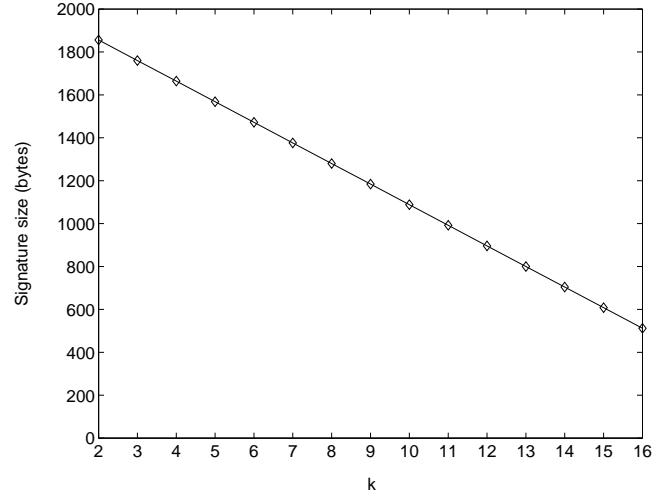
Figure 9 Signature size as a function of k .
