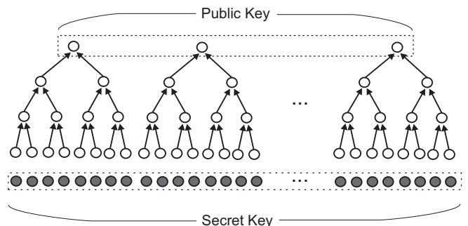
Figure 3 Public key construction using Merkle trees.
